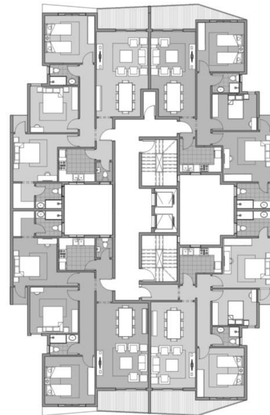
FIFTH FLOOR PLAN
