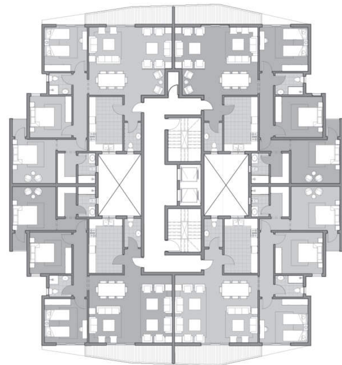
SIXTH FLOOR PLAN
