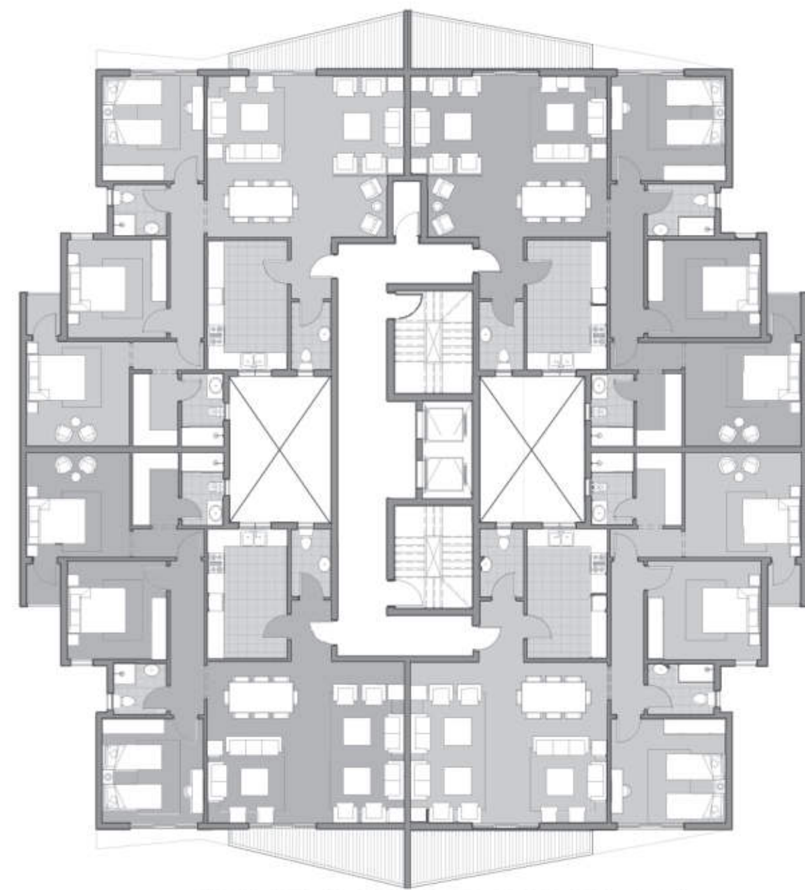
SEVENTH FLOOR PLAN
