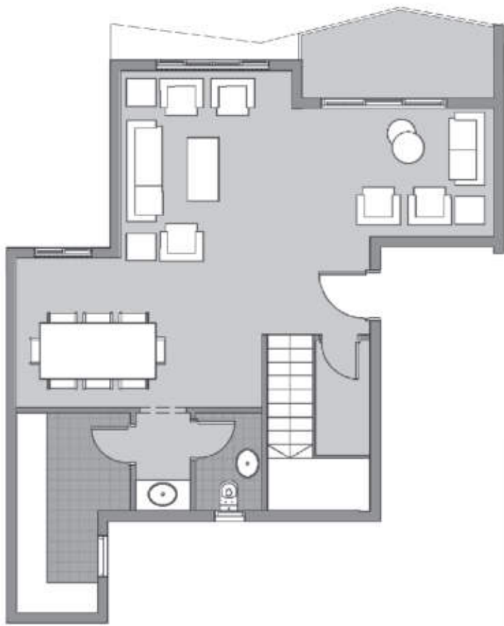
UNIT-T03 DUPLEX LOWR FLOOR
