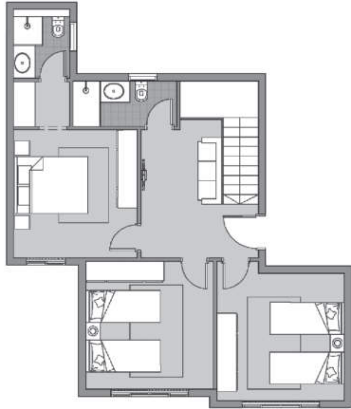
Dejoya 4 Type -E Fifth Floor Plan GROSS AREA= 194 SQ.METER
