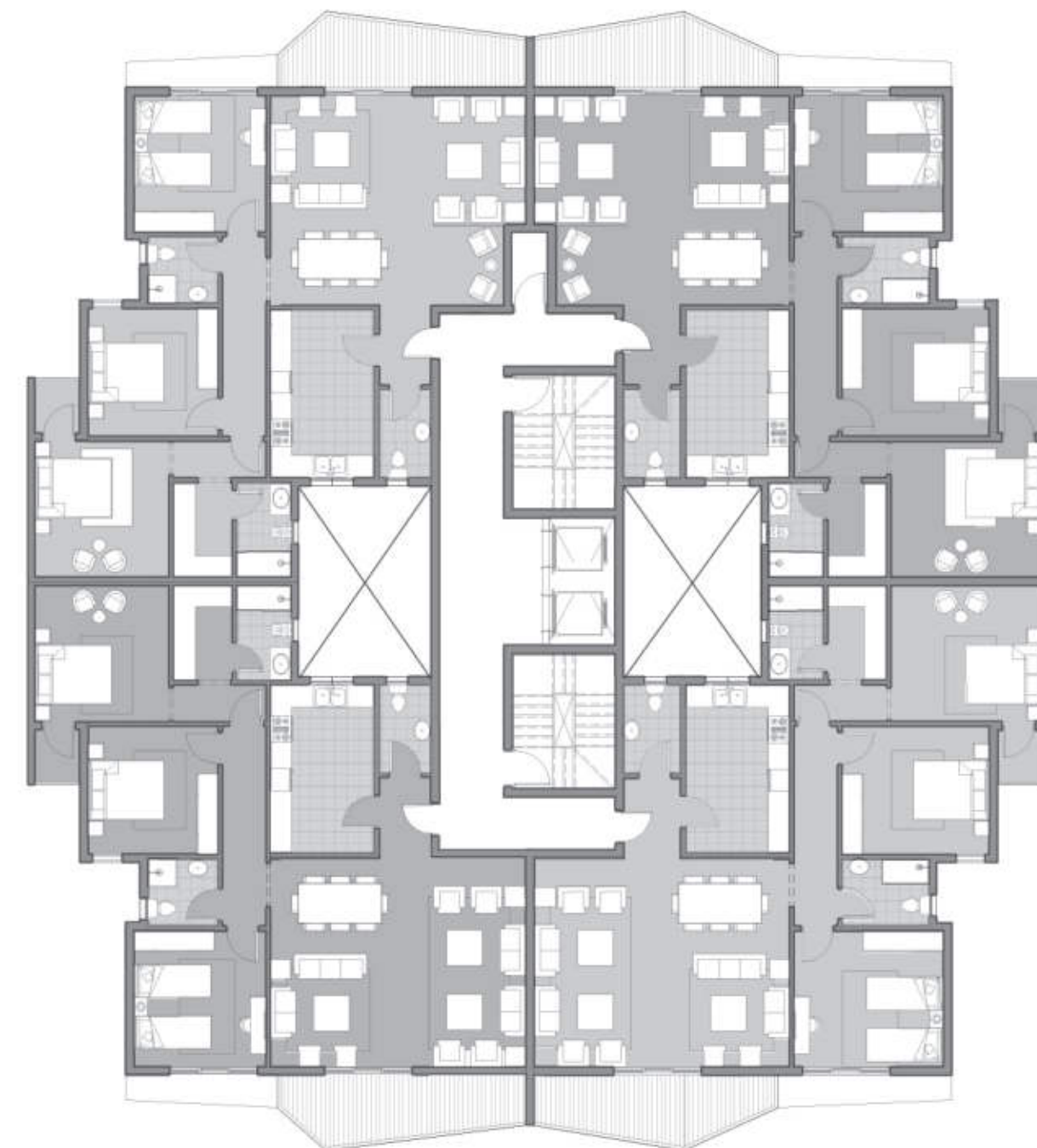
FIFTH FLOOR PLAN
