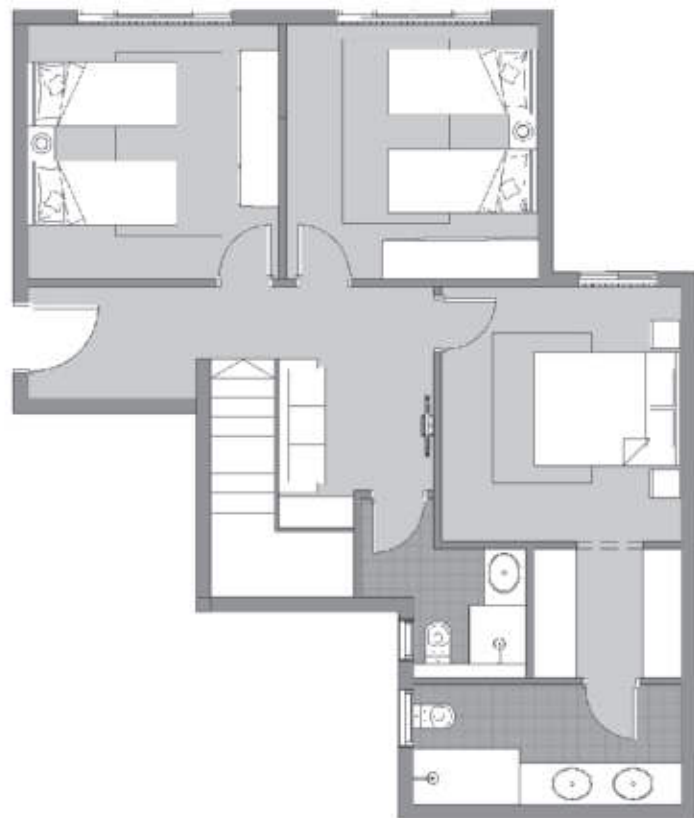
UNIT-T02 DUPLEX UPPER FLOOR
