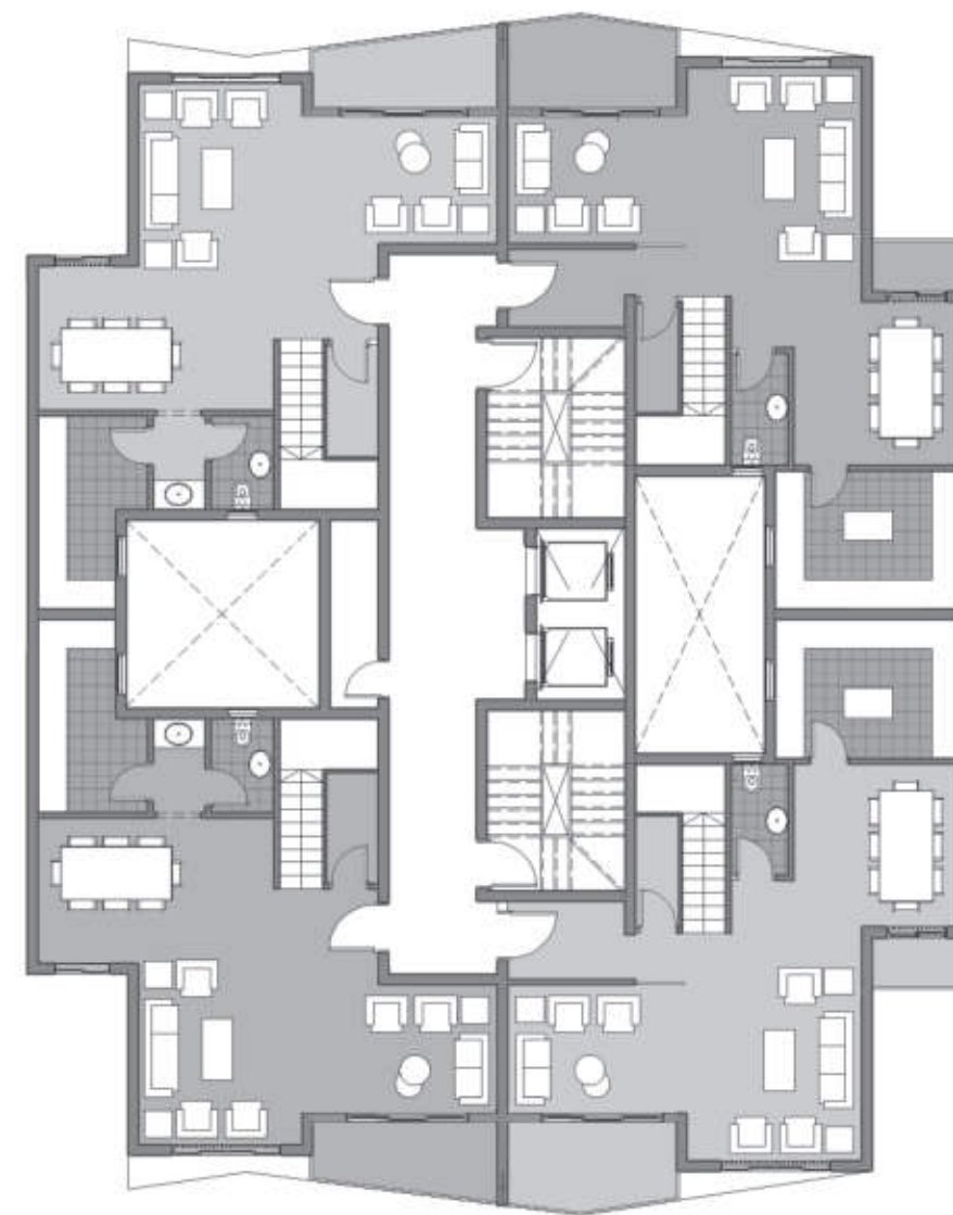
SIXTH FLOOR PLAN
