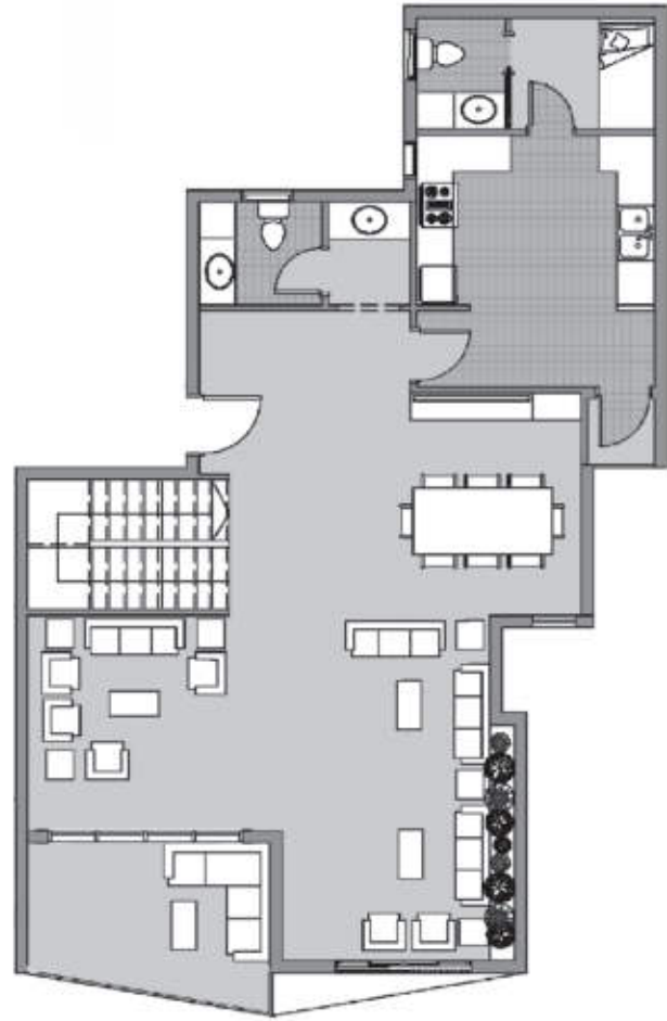
UNIT-D01 DUPLEX LOWER FLOOR
