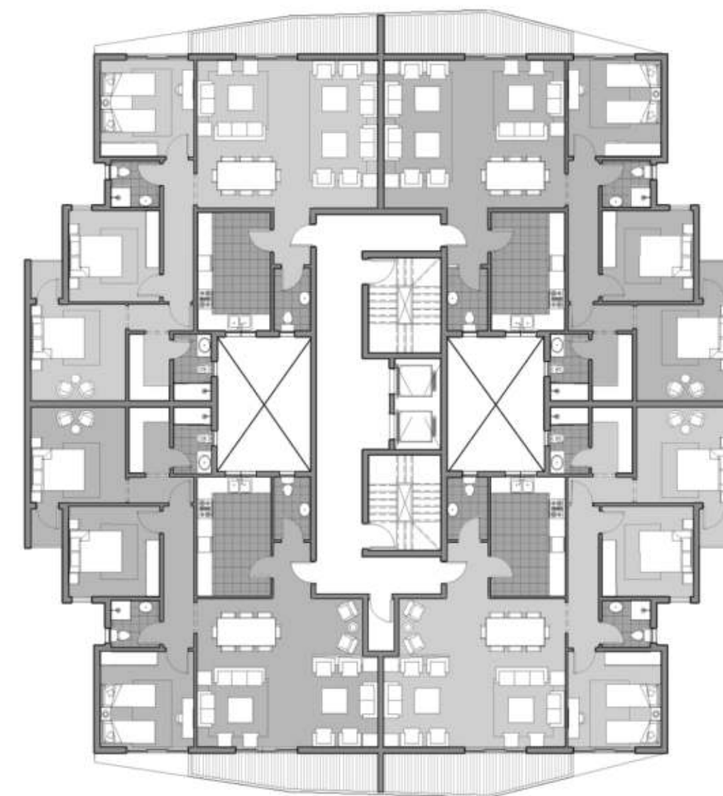
SIXTH FLOOR PLAN
