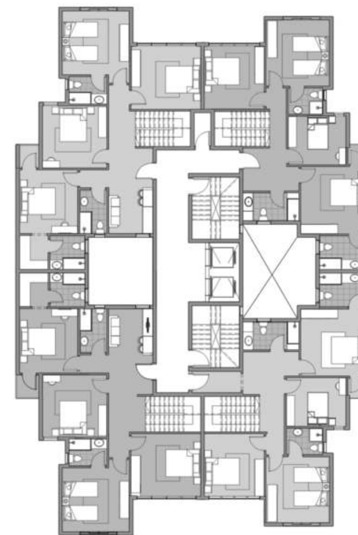
SEVENTH FLOOR PLAN
