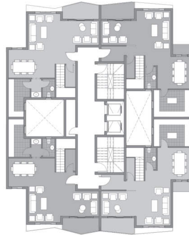
FOURTH FLOOR PLAN
