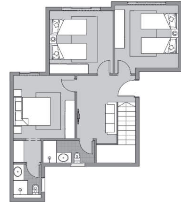
UNIT-T03 DUPLEX UPPER FLOOR
